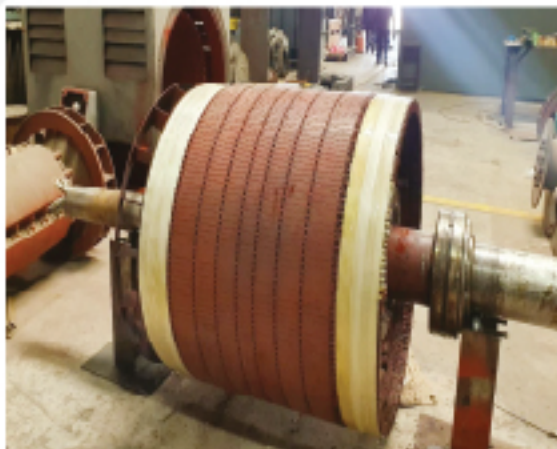
6.6 KV - 1000 KW ROTOR RE-WINDING
