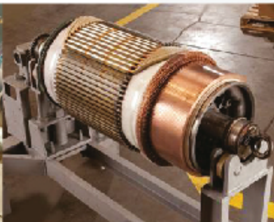
1000 HP - DC ARMATURE & STATOR RE-WINDING
