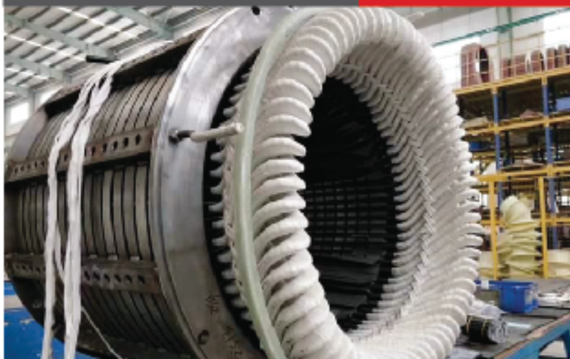
2000 KW STATOR 13.8 KV
